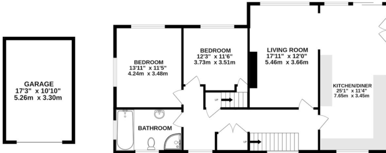
FIRST FLOOR 1275 sq.ft. (118.4 sq.m.) approx.
