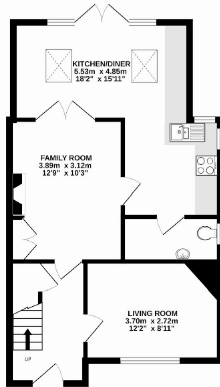
GROUND FLOOR 51.7 sq.m. (557 sq.ft.) approx.
