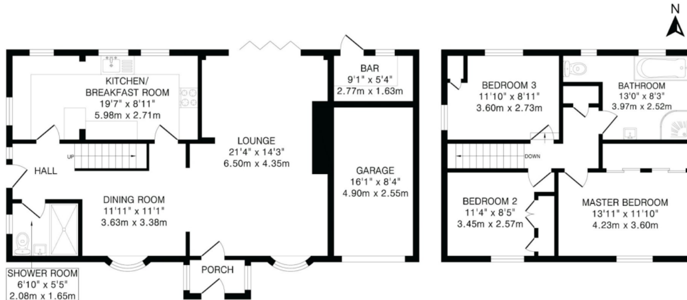
Ground Floor 929 sq.ft.(86.2 sq.m)approx.
