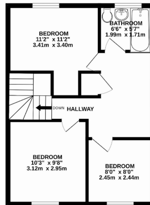
1ST FLOOR 430 sq.ft. (39.9 sq.m.) approx.
