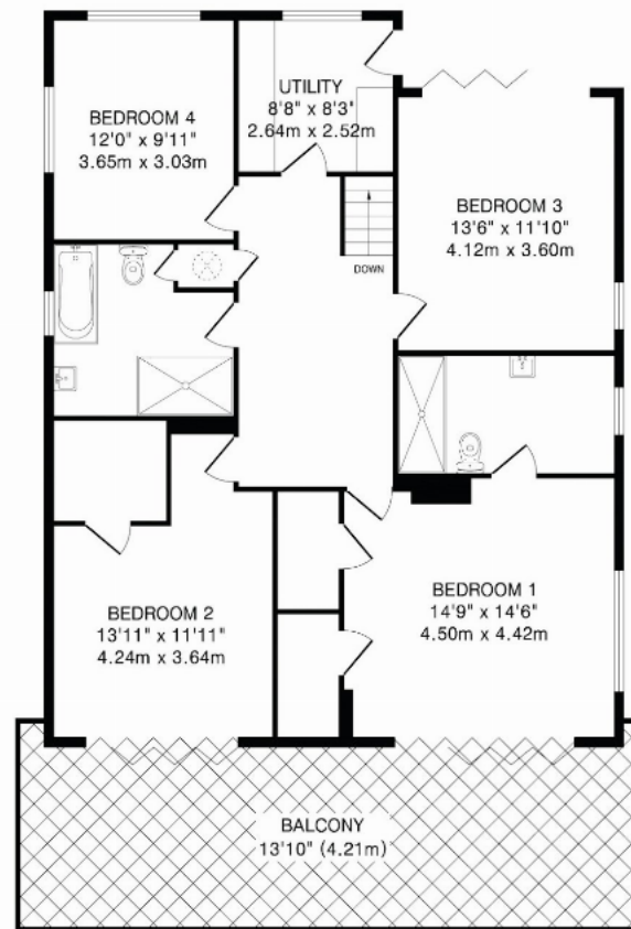
First Floor 1148 sq.ft.(106.6 sq.m)approx.
